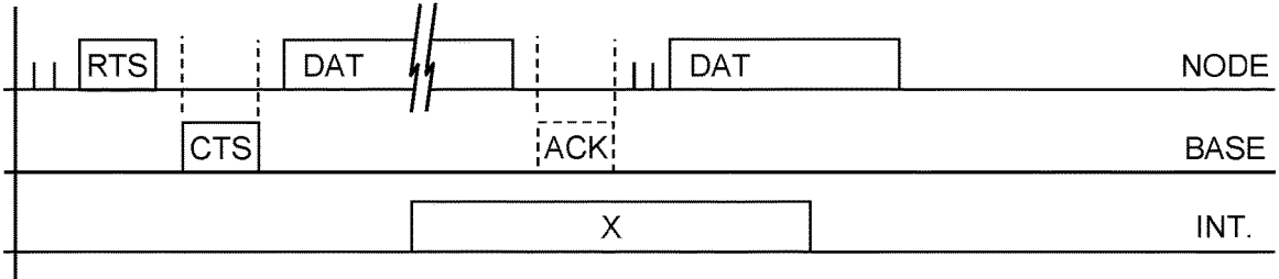
FIG. 3C (PRIOR ART)
